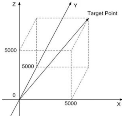
Continuous interpolation
